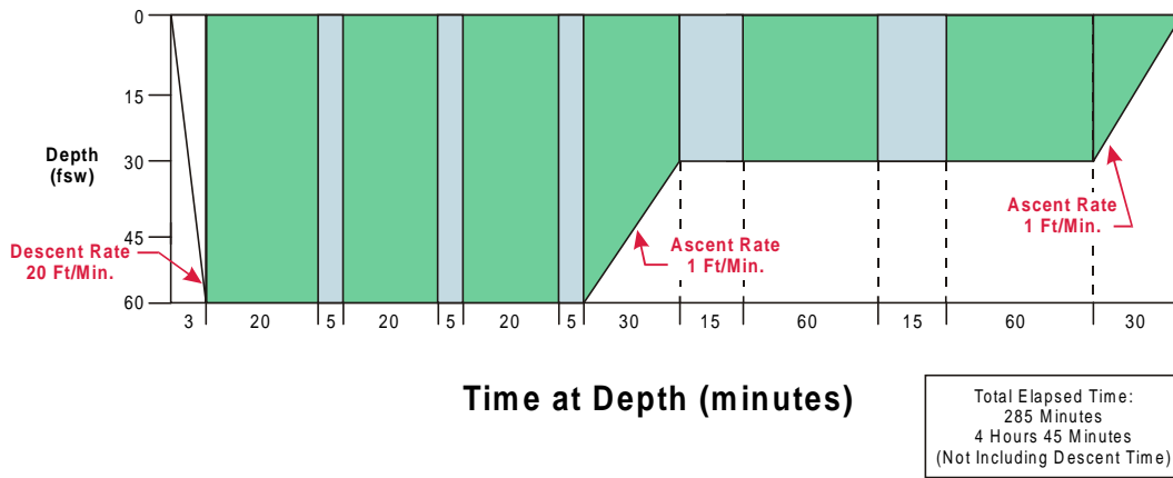
Figure 21-8. Treatment Table 6.
